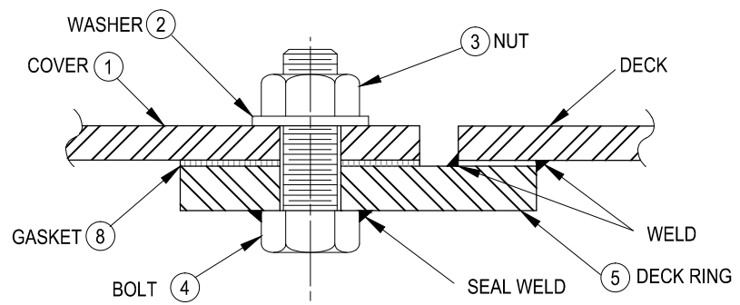
BOLT DETAIL
