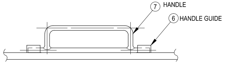
HANDLE DETAIL
