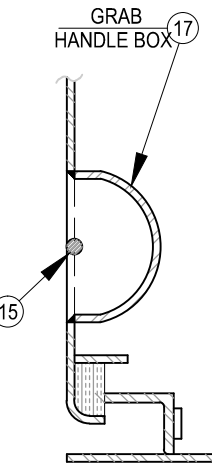
SECTION 'X-X'
