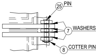
DETAIL OF DOUBLE HINGE
